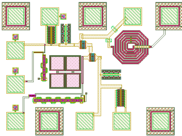
Figure 6. Layout of LNA
